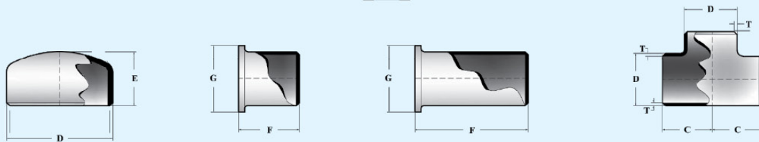
CAP (B 16.9) STUB ENDS (MSS SP 43) (SHORT NECKI) STUB ENDS (B 16.9) (LONG NECKI) EQUAL TEE (B 16.9)
